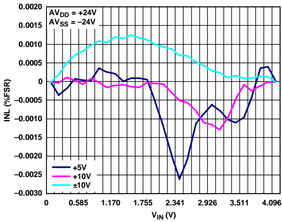
Figure 5. Integral Nonlinearity Error vs. V_{IN}
