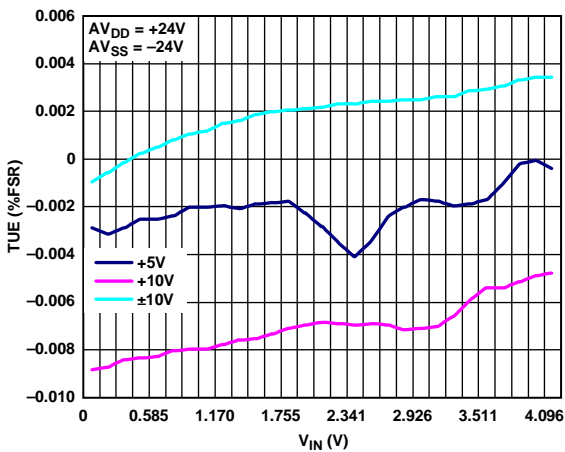
Figure 7. Total Unadjusted Error vs. V_{IN}
