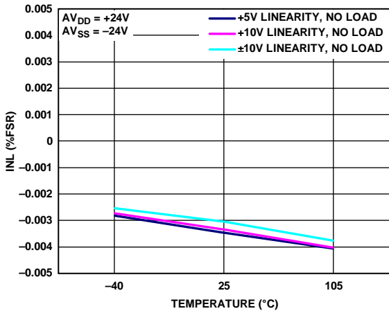
Figure 6. Integral Nonlinearity Error vs. Temperature
